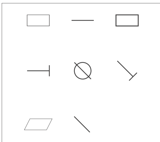
Fig. 3c: QaDiPF-Example (Schwank, 1998)
